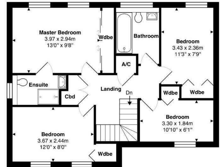
1st Floor Approx. Gross Internal Area 58.9 m 2 ... 634 ft 2
