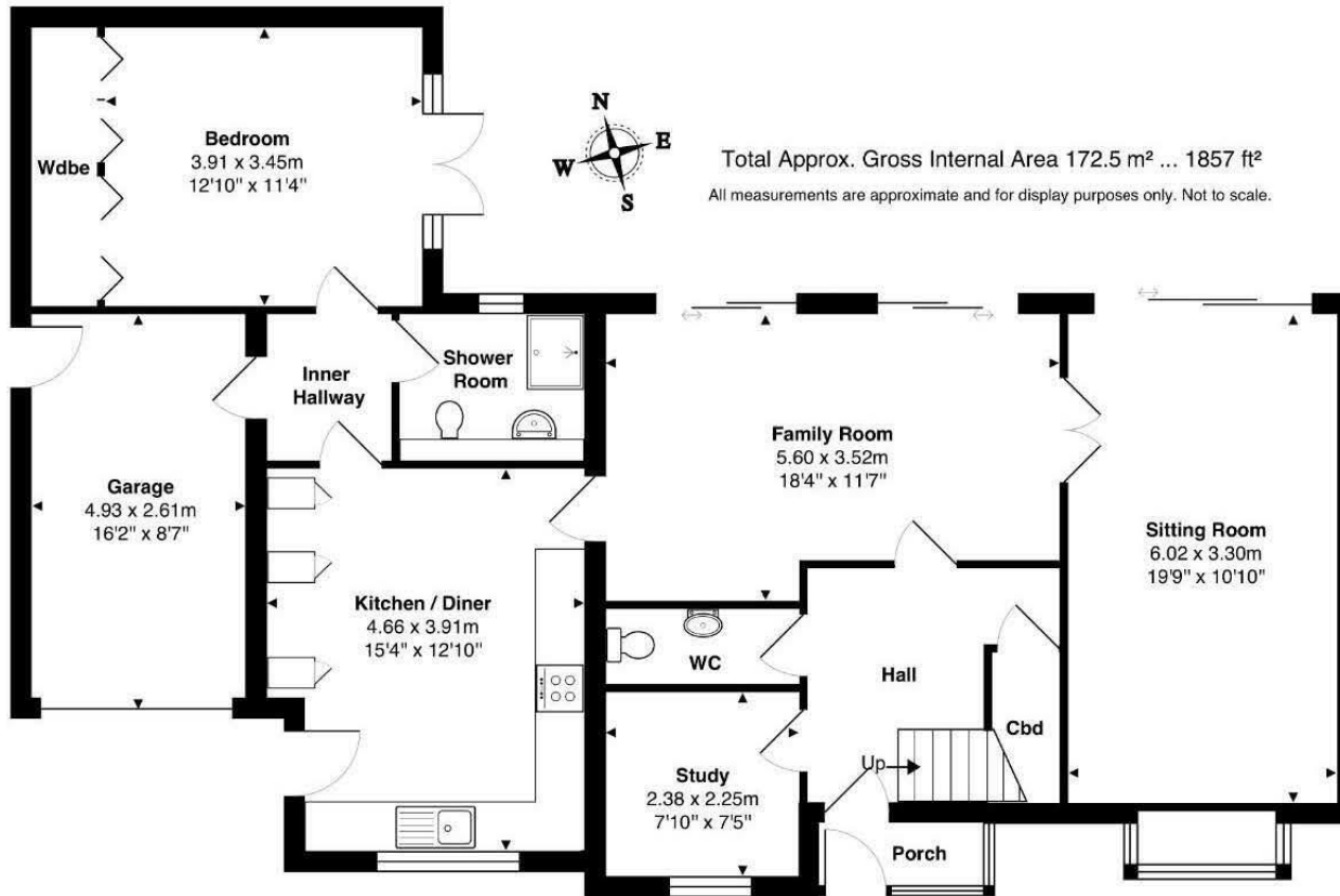
Ground Floor Approx. Gross Internal Area 113.6 m 2 ... 1222 ft 2
